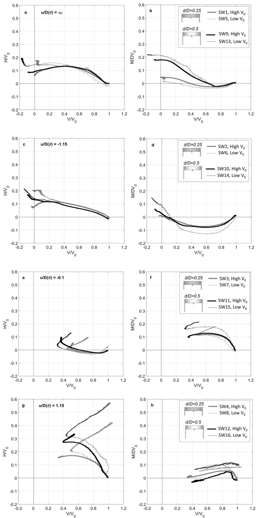
Fig. 12. Results of all swipe tests in the a) H/V_0 vs V/V_0 , b) M/DV_0 vs V/V_0 planes.
