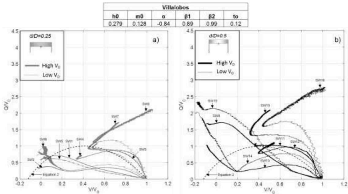
Fig. 16. Experimental results with VHM yield surface, overall fit for Villalobos parameters (2006), a) d/D = 0.25 , b) d/D = 0.5 .
