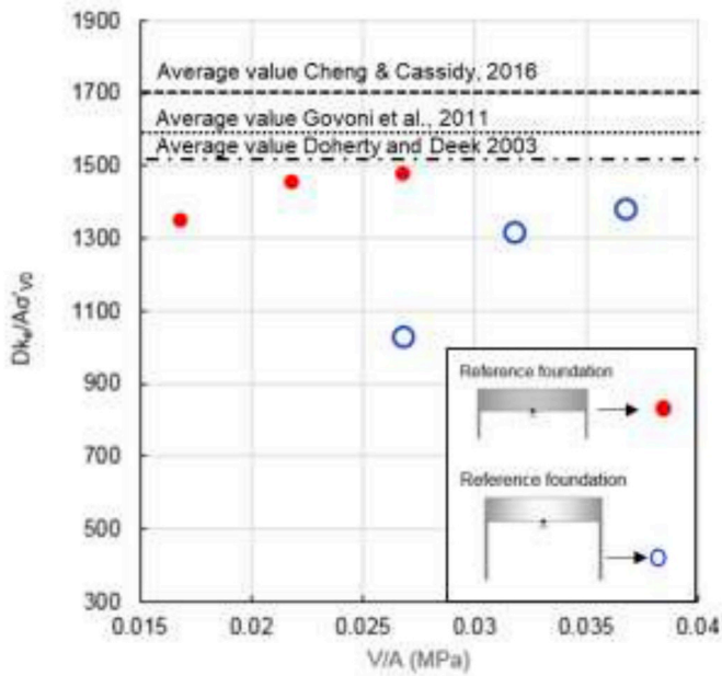
Fig. 7. Vertical unloading stiffness.
