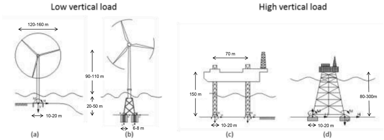
Fig. 1. Offshore energy infrastructure supported by skirted foundations as a) monopod, b and d) jacket with multiple foundations, c) jack-up with typically three foundations.
