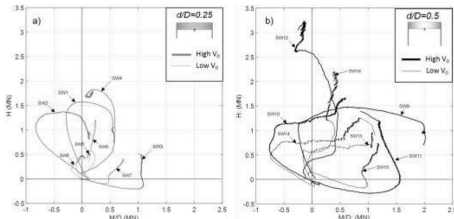
Fig. 13. Result of all swipe tests in the M/D vs H plane in prototype units for a) d/D = 0.25 and b) d/D = 0.5 .
