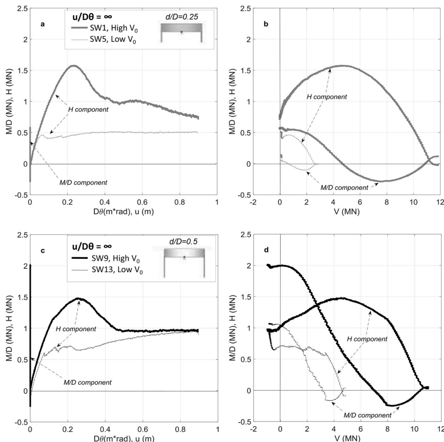
Fig. 10. Swipe test results for a test dominated by horizontal load.
