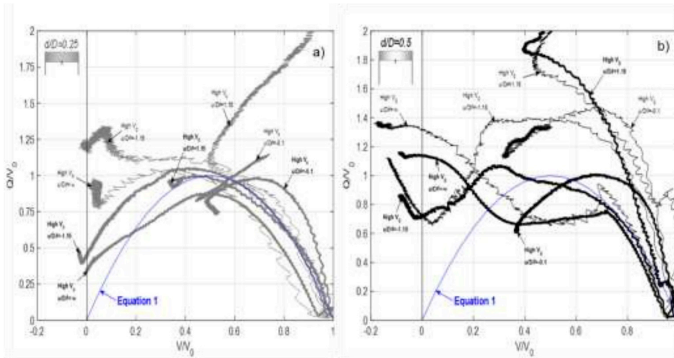
Fig. 17. Experimental results with VHM yield surface (overall fit), a) d/D = 0.25 , b) d/D = 0.5 .
