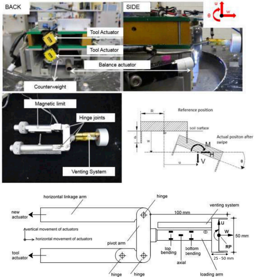
Fig. 3. Centrifuge set-up, foundation model and sign convention.
