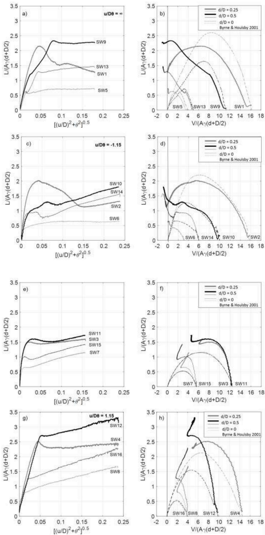
Fig. 14. Result of all swipe tests in the a) [(u/D)^2 + \theta^2]^{0.5} vs L/A\gamma(d+D/2) , b) V/A\gamma(d+D/2) : L/A\gamma(d+D/2) plane, compared with eq. (1) for surface foundations (Byrne and Housby, 2001).
