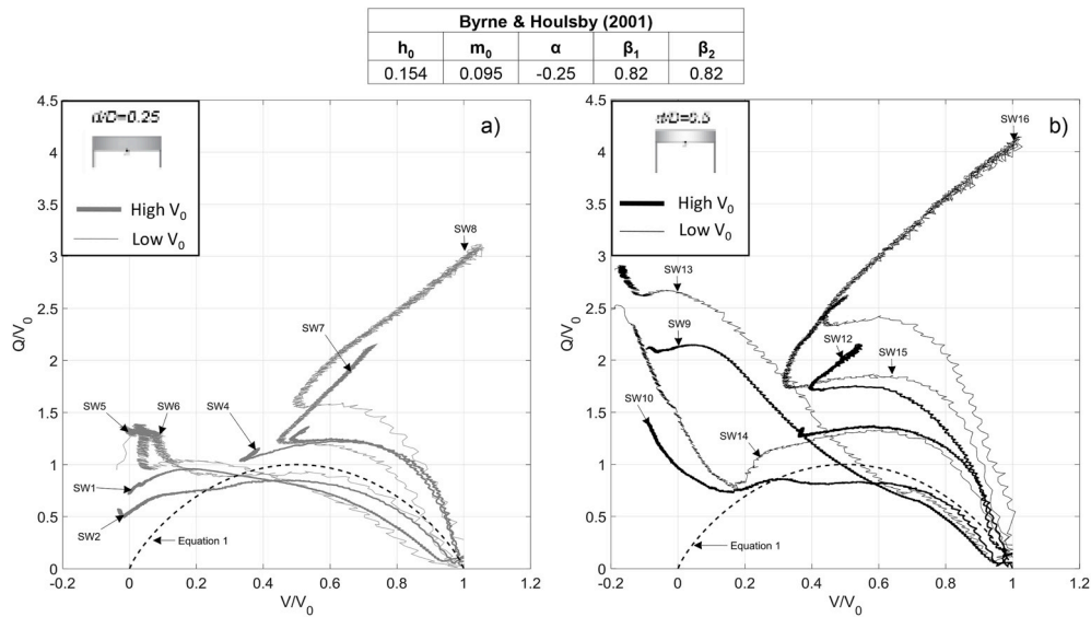
Fig. 15. Experimental results with VHM yield surface, overall fit for Housby and Byrne parameters (2001), a) d/D = 0.25 , b) d/D = 0.5 .
