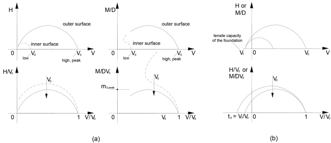
Fig. 2. Schematic representations of the yield surface for skirted foundations on sand in drained conditions based on 1 g experiments: a) shape and size governed by the mobilised stress level and M/(HD) ratio and b) allowance for horizontal and moment capacity in the tensile range of vertical load.
