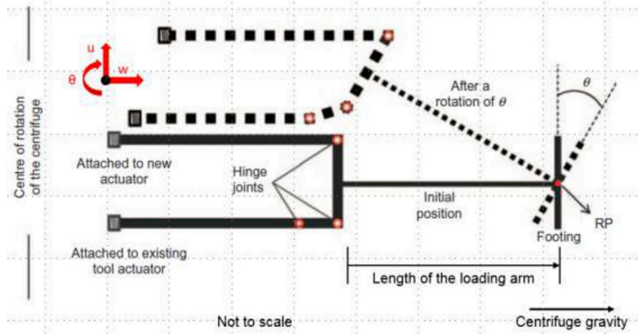
Fig. 4. Movements of the VHM actuator that result in rotation about the reference point (RP) after Zhang et al. (2013).
