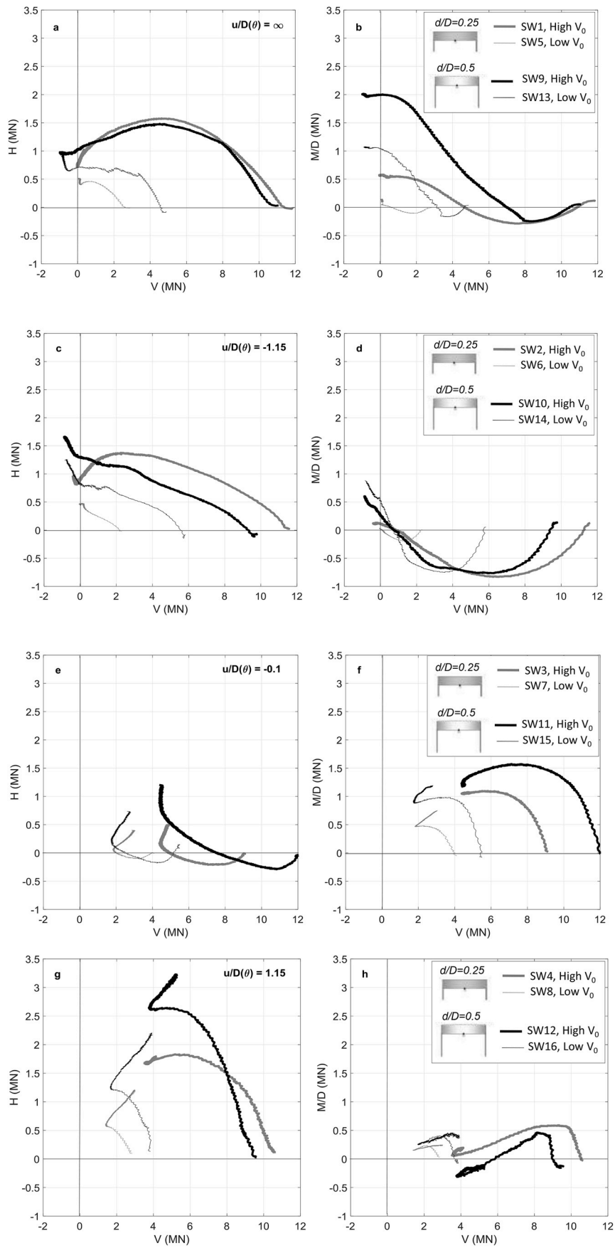
Fig. 11. Results of all swipe tests in the a) VH, b) VM/D planes.
