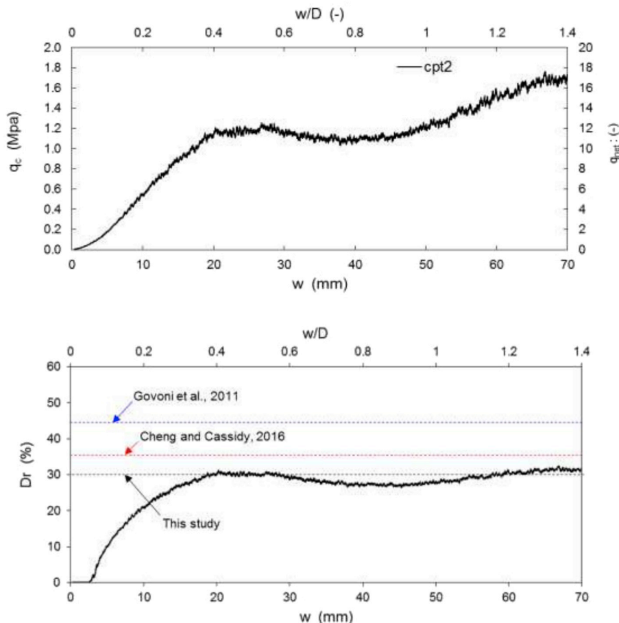
Fig. 5. Characterization of sand sample from miniature CPT, in terms of a) measured and net cone resistance, q_c and q_{net} and b) relative density D_r .
