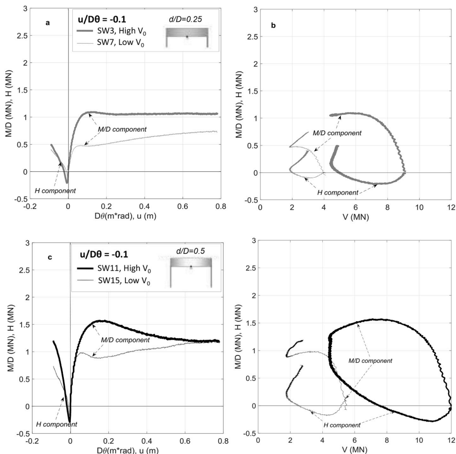
Fig. 9. Swipe test results for a test dominated by moment.
